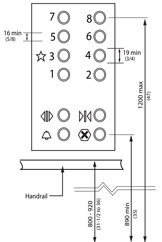
Figure 4.1.14.2 Control Panel
