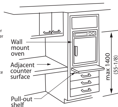
Figure 4.3.18.8 Wall-Mounted Oven
