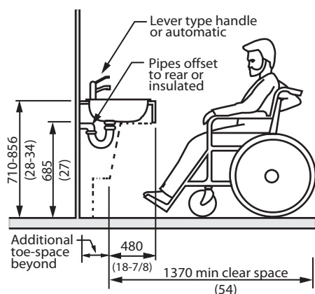
Figure 4.3.18.5 Kitchen Sink
