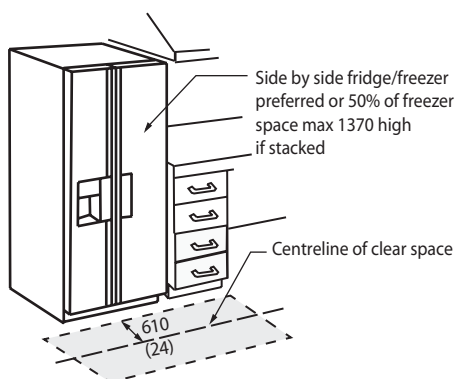
Figure 4.3.18.7 Fridge/Freezer
