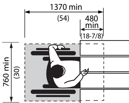
Figure 4.3.7.2 Frontal Approach
