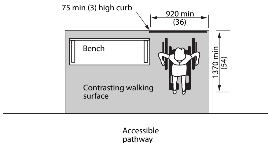
Figure 4.3.15.1 Rest Area
