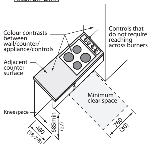
Figure 4.3.18.6 Cook Top
