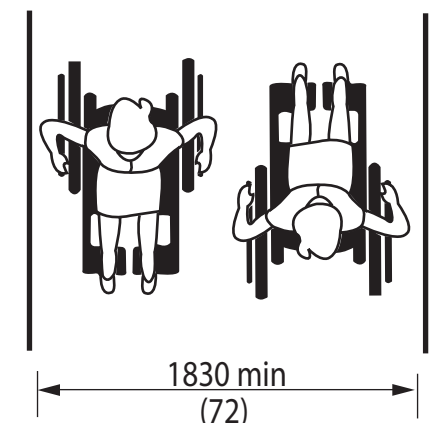
Figure 4.1.4.2 Access Widths
